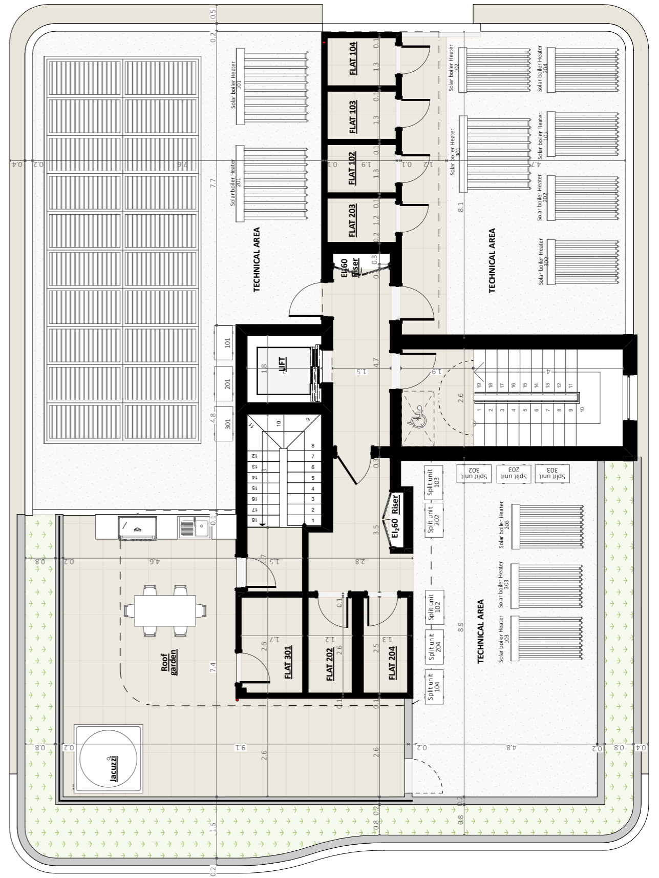
ROOF GARDEN
